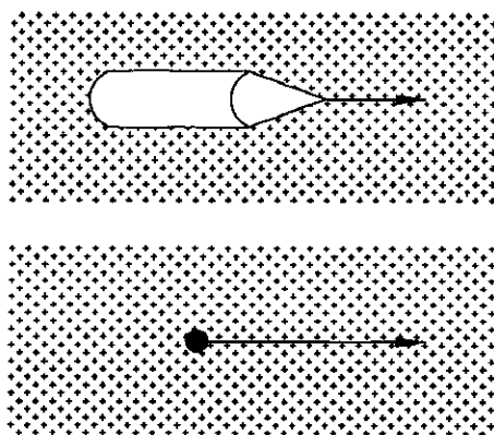
Figure 1.3. Another illustration of the second scientific imbalance studied in this monograph, the impossibility of reducing nature to point-like elementary constituents. The top view depicts a typical open nonconservative and irreversible Newtonian system with nonlocal and nonpotential forces, such as a missile moving in atmosphere, while the bottom view depicts its reduction to point-like constituents. Such a reduction is now known to be inconsistent because no finite ensemble of elementary quantum particles can reproduce a missile in atmosphere, evidently because the former system is closed, reversible and conservative, while the latter system is open nonconservative and irreversible. This establishes that the nonlinear, nonlocal and nonpotential interactions responsible for classical Newtonian systems such as a missile in atmosphere originate at the level of the ultimate elementary constituents of nature.
