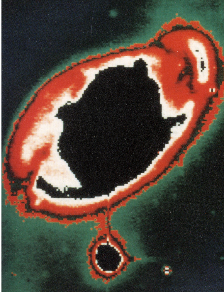
Figure 5: The experimentally verified [68] physical connection between the galaxy NGC (top) 4319 and the quasar Mark 205 (bottom), via the superposition of several gamma spectroscopic plates. By contrast, the quasar Mark 205 has a redshift with z = 0.07 , while the associated galaxy NCG 4316 has a redshift of only z = 0.0056 . The interpretation of this difference requires necessary departures from the special and general relativities, because such a large difference would require that the quasar has at least 104 times the speed of the galaxy, under which conditions the quasar and its associated galaxy would have separated completely billions of years ago. Santilli's isorelativity permits an exact, numerical, and invariant representation of the indicated large difference in cosmological redshifts, even at the limit of no relative motion with respect to Earth (picture from ref. [68]).
