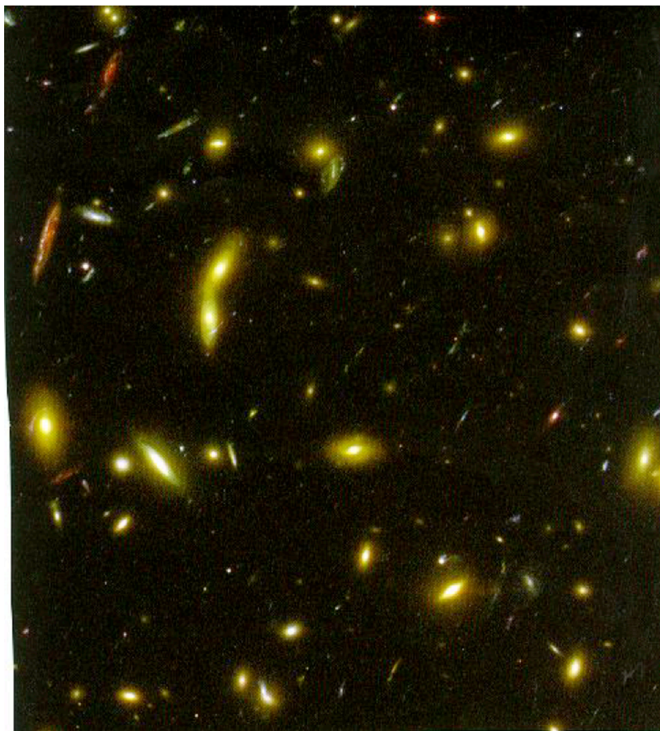
Figure 1: The 20th century astrophysics and cosmology assumed that intergalactic space is empty, thus being described by Minkowski spacetime and special relativity. In this paper, we point out that the entire universe can be seen from each of its points. But light carries energy, thus causing a local energy density. Consequently, intergalactic space is a true physical medium of low density causing a decrease of the speed of light that increases with the distance, thus eliminating the expansion of the universe and its increase with the distance.
