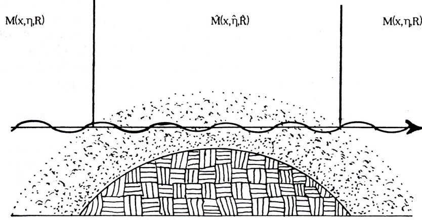
Figure 4: A schematic view of the conditions of applicability of the Minkowski-Santilli isospacetime, that within physical media such as Earth's atmosphere, while recovering uniquely and identically the conventional Minkowski spacetime in vacuum.
