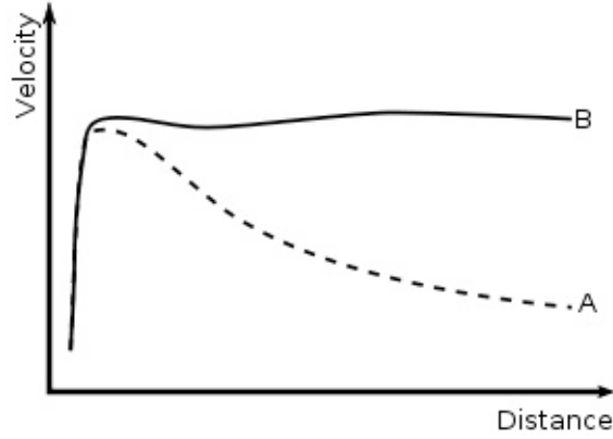
Figure 3: The deviation of the observed behavior of the speed of stars in a spiral galaxy (B) from that predicted from Newtonian gravitation (A) has been derived via the redshift of light. Therefore, it can be explained via a progressive decrease of the speed of light caused by the media with decreasing density from the galactic center (Figure 2).
