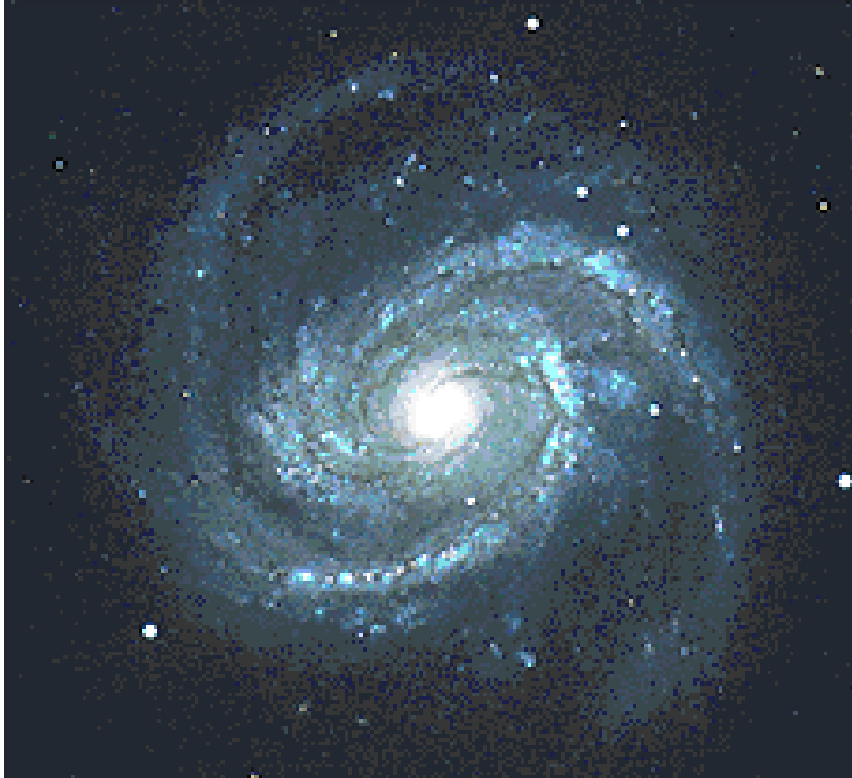
Figure 2: The 20th century astrophysics and cosmology assumed that interstellar space inside a given galaxy is empty, thus verifying special relativity. In this paper, we point out that space within a galaxy is filled up with matter whose density decreases with the radial distance from the center, thus causing a slowdown of the speed of light that decreases with the increase of the distance, thus eliminating the need for dark matter (see Figure 3).
