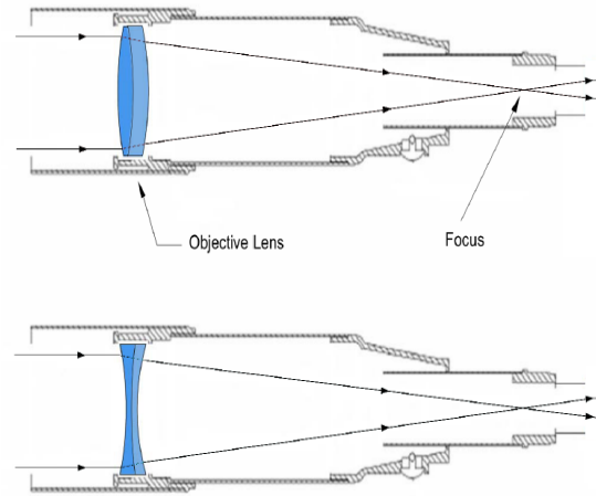
Figure 14: Schematic view of the telescopes with convex and concave lens [43].
