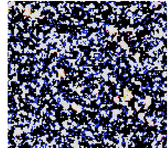
Figure 37: Picture from the Santilli telescope of a circular trace [44].
