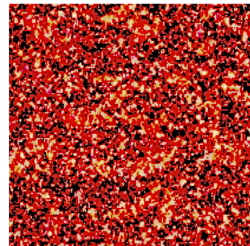
Figure 24: The first of numerous circular traces identified in a picture of Vega regions of the night sky on November 7, 2013, with the Santilli's antimatter
