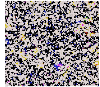
Figure 36: Picture from the Santilli telescope of an unknown event in the Epsilon sky region from Sebring, Florida [44].
