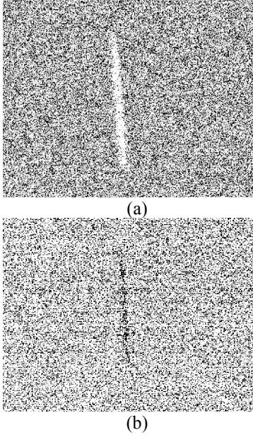
Figure 44: Images from the Vega region of the night sky showing a streak due to matter light from the Galileo telescope (a) and a streak of darkness from the Santilli telescope caused by antimatter light (b) [47].
