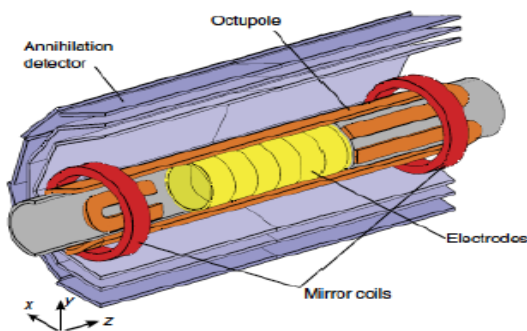
Figure 5: An illustration from Ref. [34] providing a cut-away diagram of the antihydrogen production and trapping of the ALPHA Collaboration, showing the relative positions of the cryogenically cooled Penning- Malmberg trap electrodes and other features.
