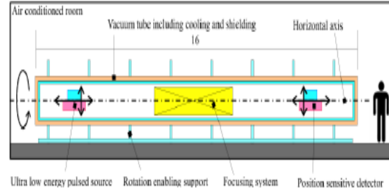
Figure 4: The possible alternatives for a collimated beam of positrons. Santilli's isodual theory of antimatter predicts gravitational repulsion (antigravity) at all its levels for positrons in a horizontal flight on Earth that, for very low energy of the order of meV, is of the order of 1 cm following a 10 m flight, thus being visible to the naked eye on the scintillator at the end of the tube. For that reason, Santilli's proposed experiment has been stated to be "resolatory" by experimentalists in the field [12, 27]. The lower two renderings are from the technical realization of the test [28] by the R. M. Santilli Foundation on the technical realization of proposal [6] (forth view from the top) and illustration of its size compared to a person [29].
