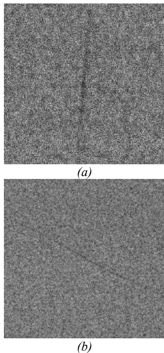
Figure 49: Images from the Draco region of the night sky showing a streak of darkness expectedly from a far away antimatter light (a), and a streak of darkness expectedly from a small antimatter asteroid annihilating in our atmosphere (b) [47].
