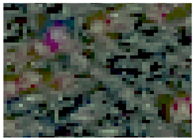
Figure 20: View of Third streak of light detected in the Epsilon Alpha and Beta region with the Santilli telescope of antimatter galaxies [43]
