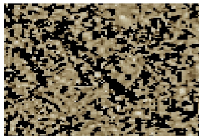
Figure 21: The first streak of darkness identified in the picture of the Epsilon Alpha and Beta region of the night sky taken with the antimatter telescope
