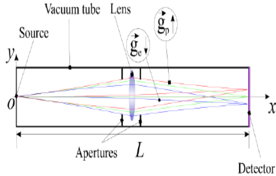
Figure 3: Principle set-up of Mills's adaptation of Santilli's comparative test of the gravity of electrons and Positrons. \rightarrow shows the gravitational attraction on a collimated beam of electrons that, when having a very low energy of the order of meV, is of the order of 1 cm following a flight of 10 m, thus being visible to the naked eye [12].
