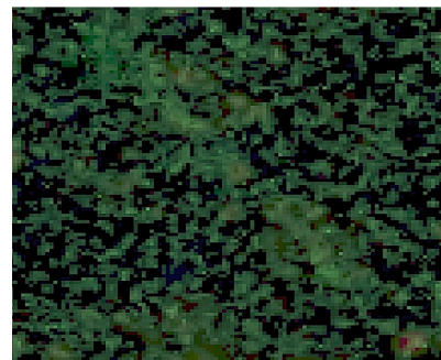
Figure 17: View of one of the streaks of matter light
