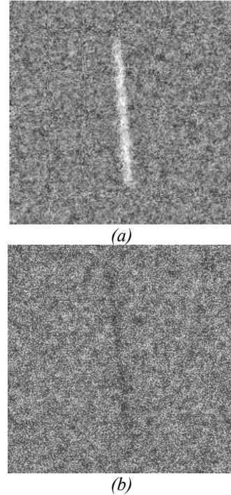
Figure 47: Images from the Draco region of the night sky showing a streak caused by matter light from the Galileo telescope (a) and a streak of darkness from the Santilli telescope caused by antimatter light (b) [47].
