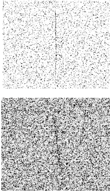
Figure 45: Images from the Vega region of the night sky from the Santilli telescope showing streaks of darkness caused by antimatter light [47].
