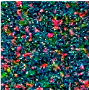
Figure 34: Picture from the Santilli telescope of a black streak in the Vega region of the sky from
