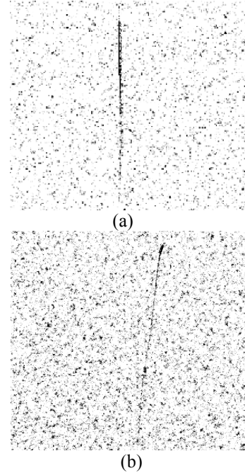
Figure 46: Images from the Vega region of the night sky showing a streak of darkness expected from a far away antimatter light (a), and a streak of darkness expected from a small antimatter asteroid annihilating in our atmosphere (b) [47].
