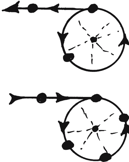
Fig. 3. A schematic view of the transformation of linear into angular motion and vice-versa that could play a crucial role in the synthesis of the neutron and its stimulated decay. Note that such a transformation is outside the capabilities of the Poincaré symmetry due to its sole validity for Keplerian systems, that is, for massive points orbiting around a heavier nucleus without collisions. By comparison, the transformation of this figure requires the presence of subsidiary constraints altering the conservation laws, thus altering the very structure of the applicable symmetry.
