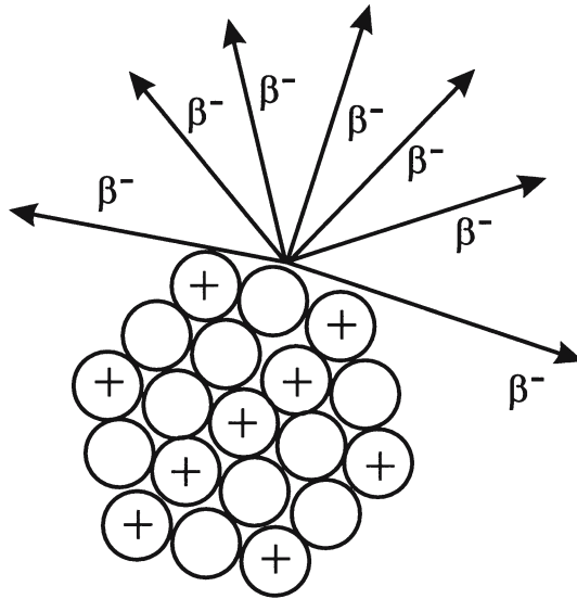
Fig. 1. A conceptual illustration of the expected dependence of the kinetic energy of the electron in nuclear beta decays on the direction of emission due to the strongly attractive Coulomb interaction between the positively charged nucleus and the negatively charged electron.
