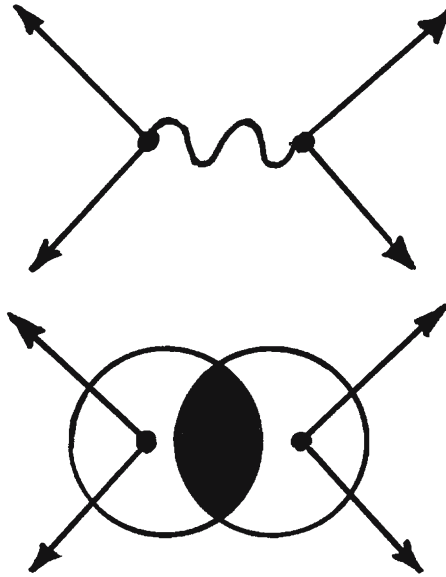
Fig. 2. A schematic illustration of the lack of established validity of the conventional (quantum) scattering theory in the elaboration of neutrino experiments due to the abstraction of all particles as massive points (top view), while particles used in neutrino experiments are extended with hyperdense medium resulting in deep overlappings and mutual penetrations (bottom view). The latter conditions require a broader scattering theory including nonlocal, nonlinear and non-Hamiltonian effects under which the claimed experimental results are not expected to remain necessarily valid.
