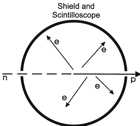
Fig. 7. A schematic view of the proposed measurement of the energy of the electron in spontaneous neutron decays to ascertain whether there is any energy left for the neutrino.
