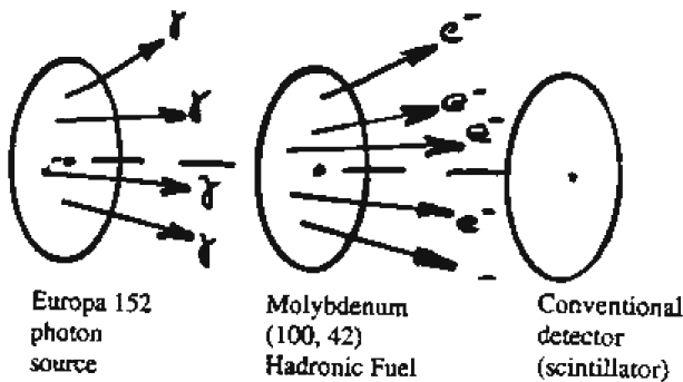
Fig. 5. The view illustrates a “hadronic fuel”, the Mo(100,42), that, when hit by a neutron resonating frequency, is predicted to experience a stimulated decay into an unstable isotope (Tc(100, 43) that, in turn, decays spontaneous into the final stable isotope Ru(100, 44) with the total emission of two highly energetic electrons. Note that the molybdenum is a conductor, hence, the predicted energy is twofold, of electric and thermal nature.
