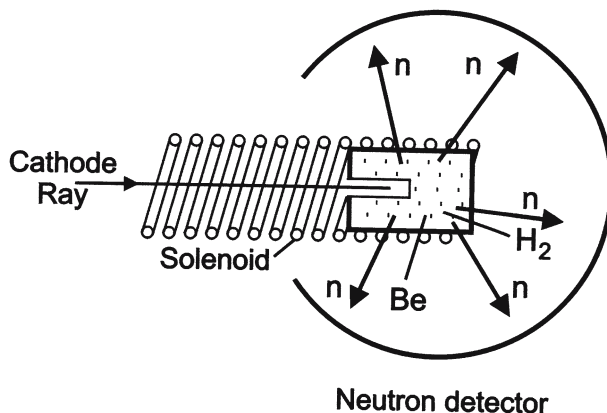
Fig. 6. A schematic view of the proposed laboratory synthesis of the neutron from protons and electrons to identify the needed energy.
