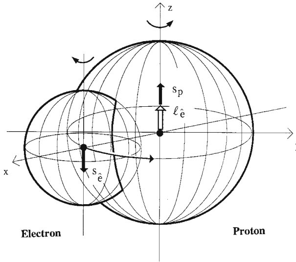
Fig. 4. A schematic view of the intrinsic and orbital angular momenta in Rutherford's synthesis of the neutron according to hadronic mechanics.
